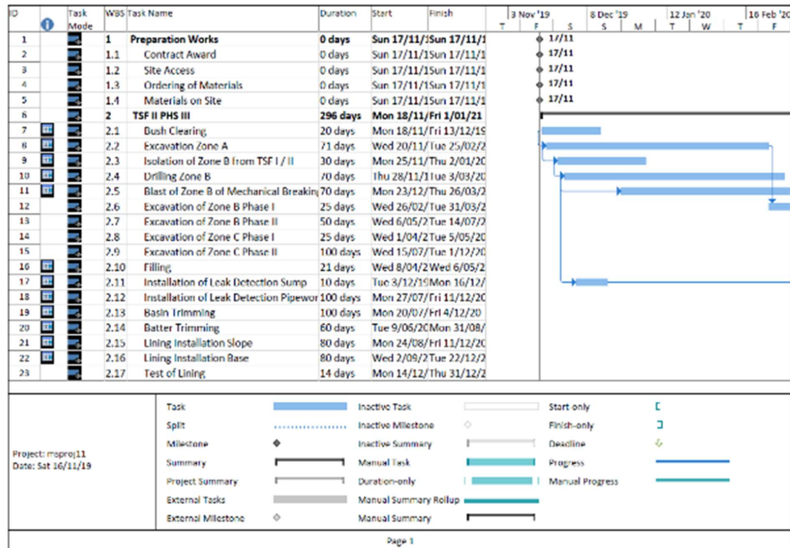
Figure 2. Construction program developed in Microsoft Project for TSF2 Phase III. The program illustrates the planned sequence of construction activities, task dependencies, procurement milestones and commissioning, providing the basis for coordinating engineering, procurement and construction activities throughout project delivery.
